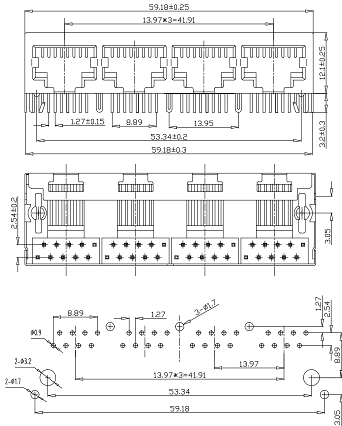
PC Board Layout Component Side Shown
