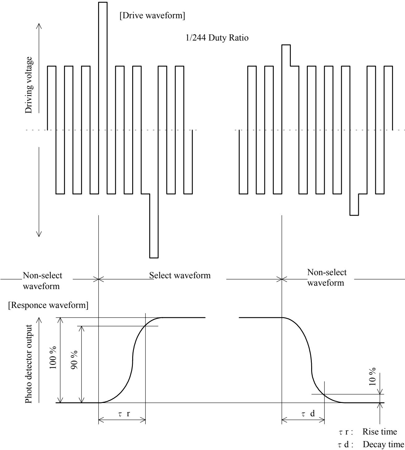
Fig.11 Definition of Response time
