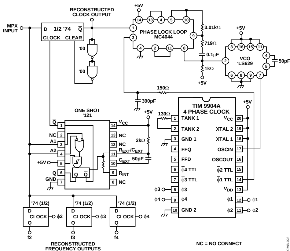
Figure 30. SVFC Demultiplexers
