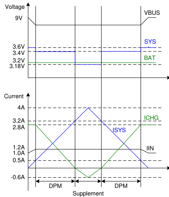
图 8-8. DPM Response
