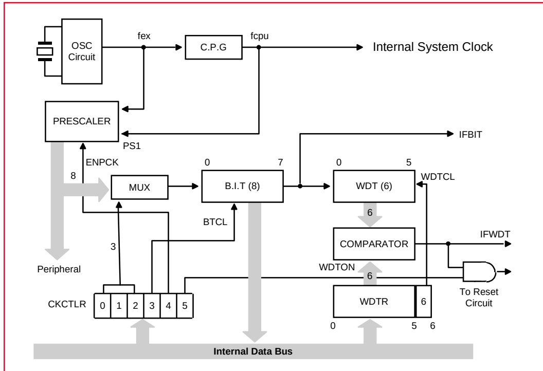
Figure 10-1 Block Diagram of Clock Generator
