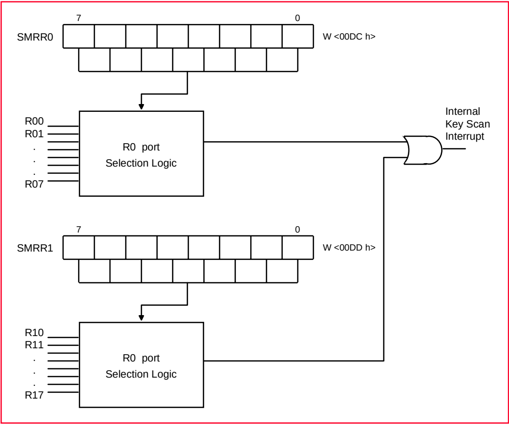
Figure 12-5 Key Scan Block
