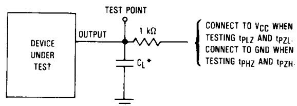
Figure 6. Test Circuit
