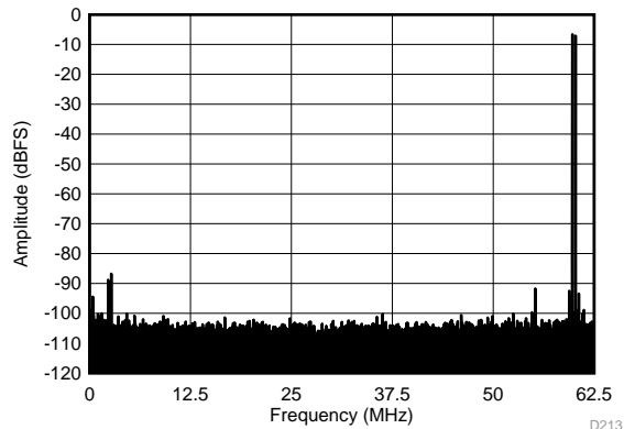
f_{IN1} = 185\text{ MHz} , f_{IN2} = 190\text{ MHz} , \text{IMD3} = 86\text{ dBFS} , each tone at -7 dBFS
