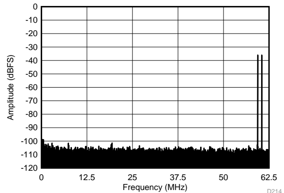
f_{IN1} = 185\text{ MHz} , f_{IN2} = 190\text{ MHz} , \text{IMD3} = 102\text{ dBFS} , each tone at -36 dBFS
