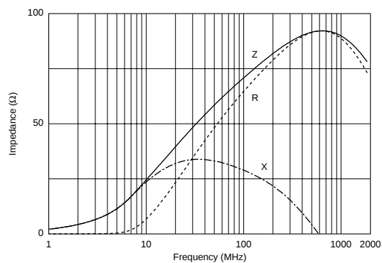
BLM18SG700TN1
