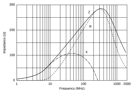
BLM18SG221TN1
