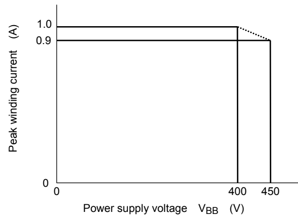
Figure 2 SOA at T_c = 95^\circ\text{C}
