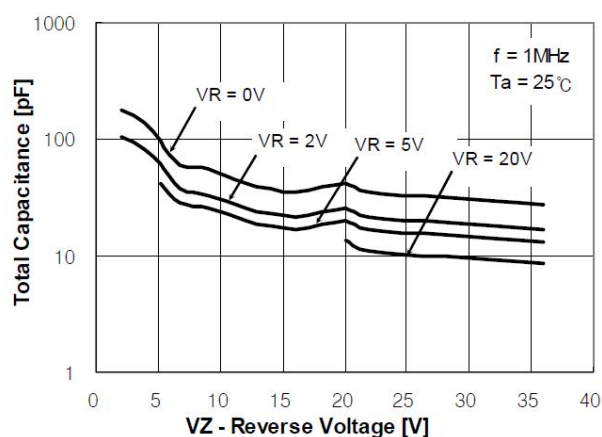
Figure 2. Total Capacitance
