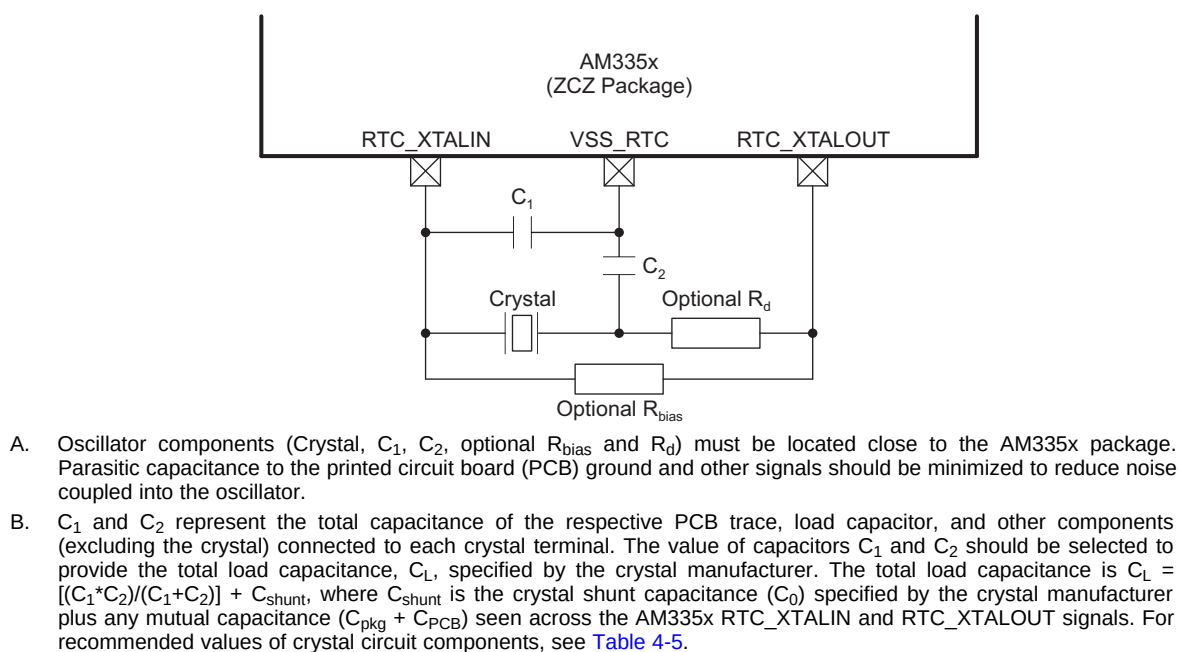
Figure 4-12. OSC1 (ZCZ Package) Crystal Circuit Schematic
