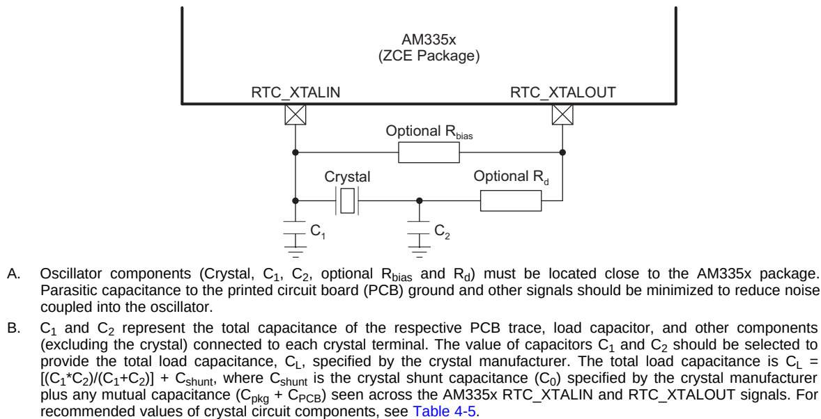
Figure 4-11. OSC1 (ZCE Package) Crystal Circuit Schematic
