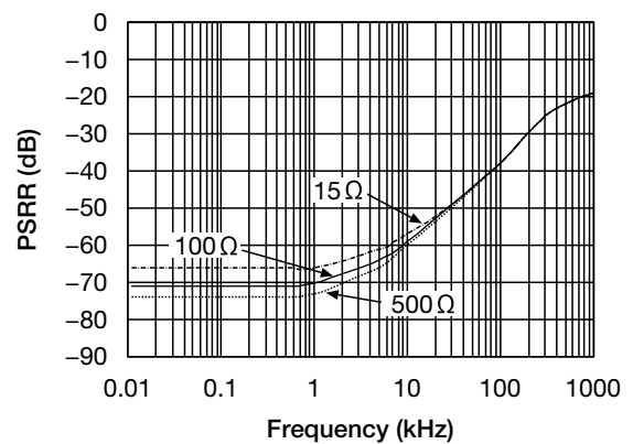
■ Ripple Rejection
