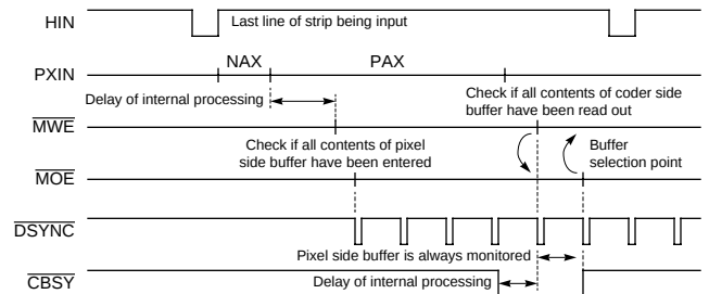
Figure 25. Compression Operation When \overline{\text{CBSY}} is Asserted but the Line is not Ignored
