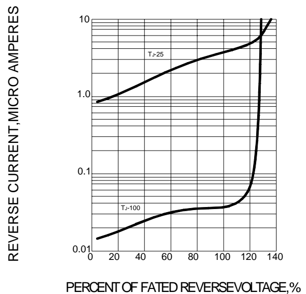
FIG.5–TYPICAL REVERSE CHARACTERISTICS
