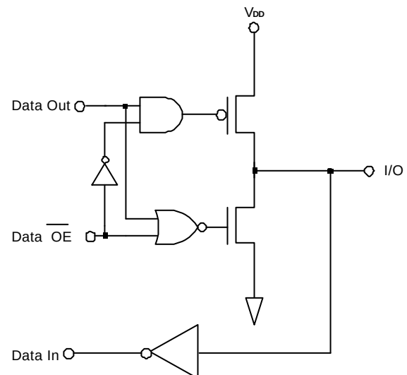
Figure 12.5. I/O Structure
