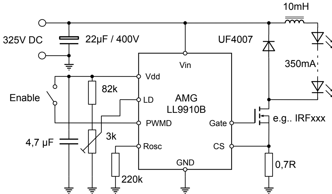
Figure4: Buck topology, linear dimming, enable switch
