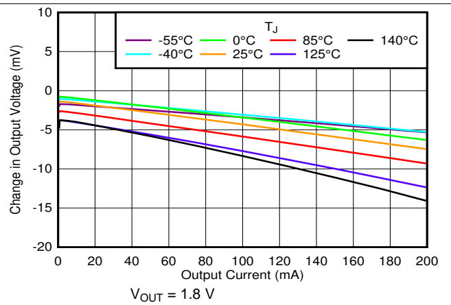
Figure 32. Load Regulation vs V_{IN} and Temperature
