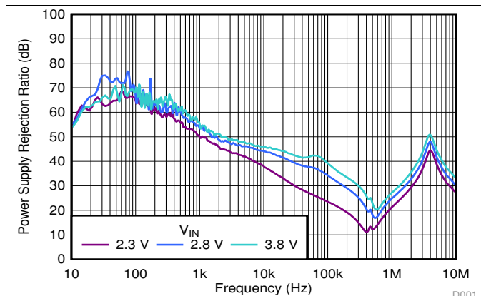
Figure 45. PSRR vs Frequency and V_{IN}
