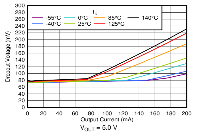
Figure 34. Dropout vs I_{OUT} and Temperature
