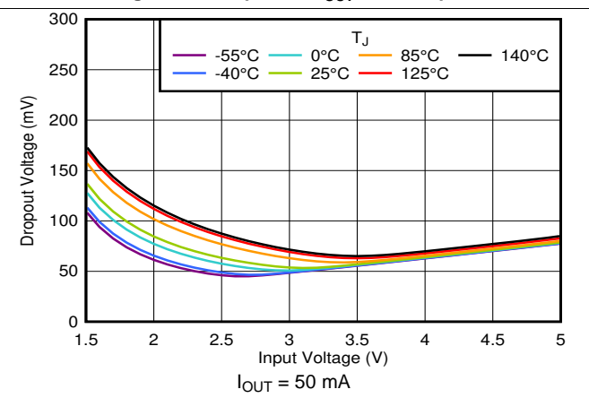
Figure 36. Dropout vs V_{IN} and Temperature
