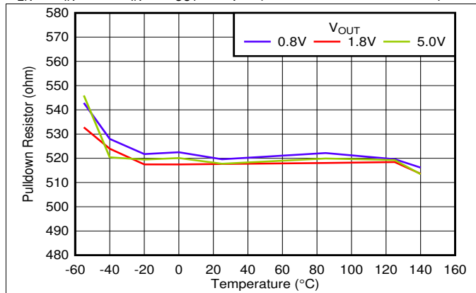
Figure 43. Smart Enable Pulldown Resistor vs Temperature and V_{OUT}
