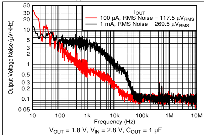
Figure 49. Output Noise vs Frequency and I_{OUT}
