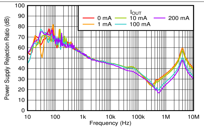
Figure 44. PSRR vs Frequency and I_{OUT}
