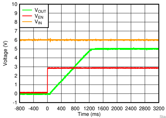
Figure 55. Startup With V_{EN} After V_{IN}
