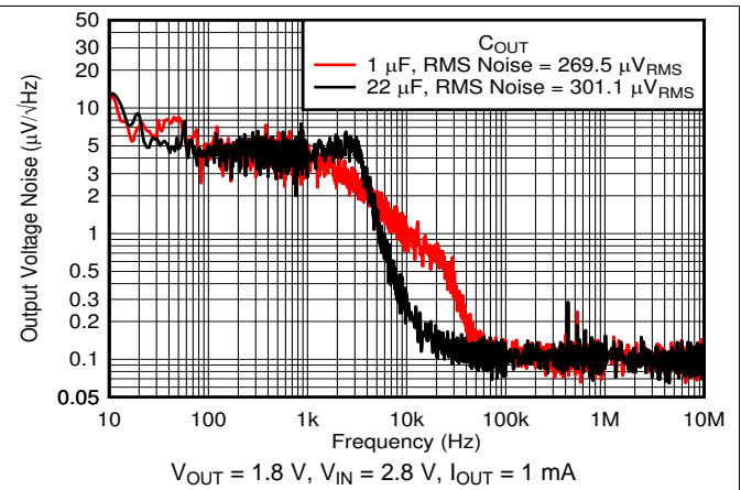
Figure 50. Output Noise vs Frequency and C_{OUT}
