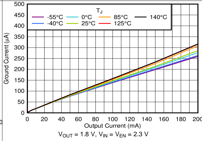
Figure 4. I_Q vs I_{OUT} and Temperature Up to 200 mA
