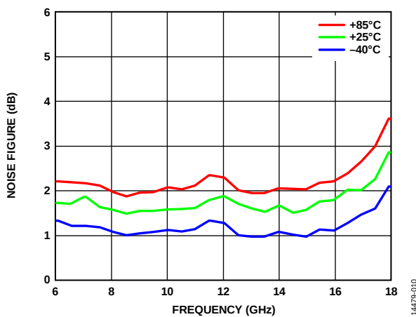
Figure 10. Noise Figure vs. Frequency for Various Temperatures (Board Loss Removed from Gain, Power, and Noise Figure Measurements)
