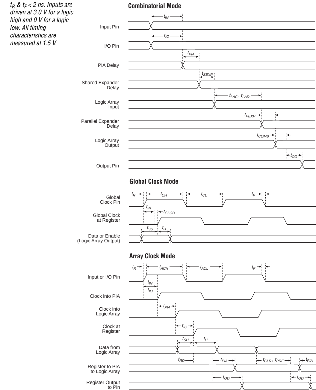
Figure 14. MAX 7000B Switching Waveforms
