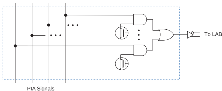
Figure 5. MAX 7000B PIA Routing
