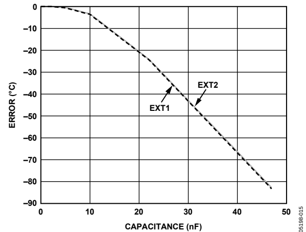
Figure 13. Remote Temperature Error vs. Capacitance Between D1+ and D1-
