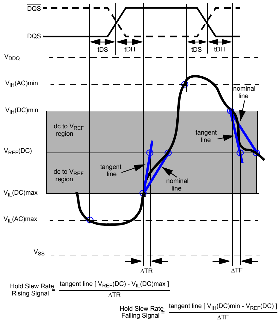
Figure 13. Illustration of tangent line for t_{\text{DH}} (differential DQS, \overline{\text{DQS}} )
