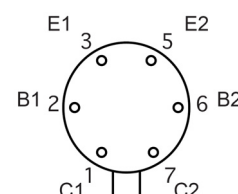
TO-71 (Bottom View)
