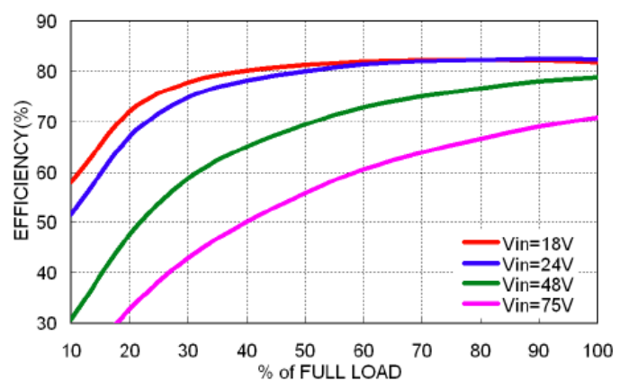
DCSDW01-48S05 Efficiency vs. Output Current
