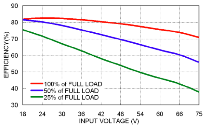
DCSDW01-48S05 Efficiency vs. Input Voltage
