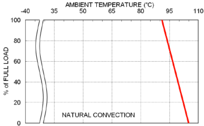
DCSDW01-48S05 Derating Curve
