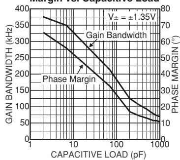
Gain Bandwidth and Phase Margin vs. Capacitive Load
