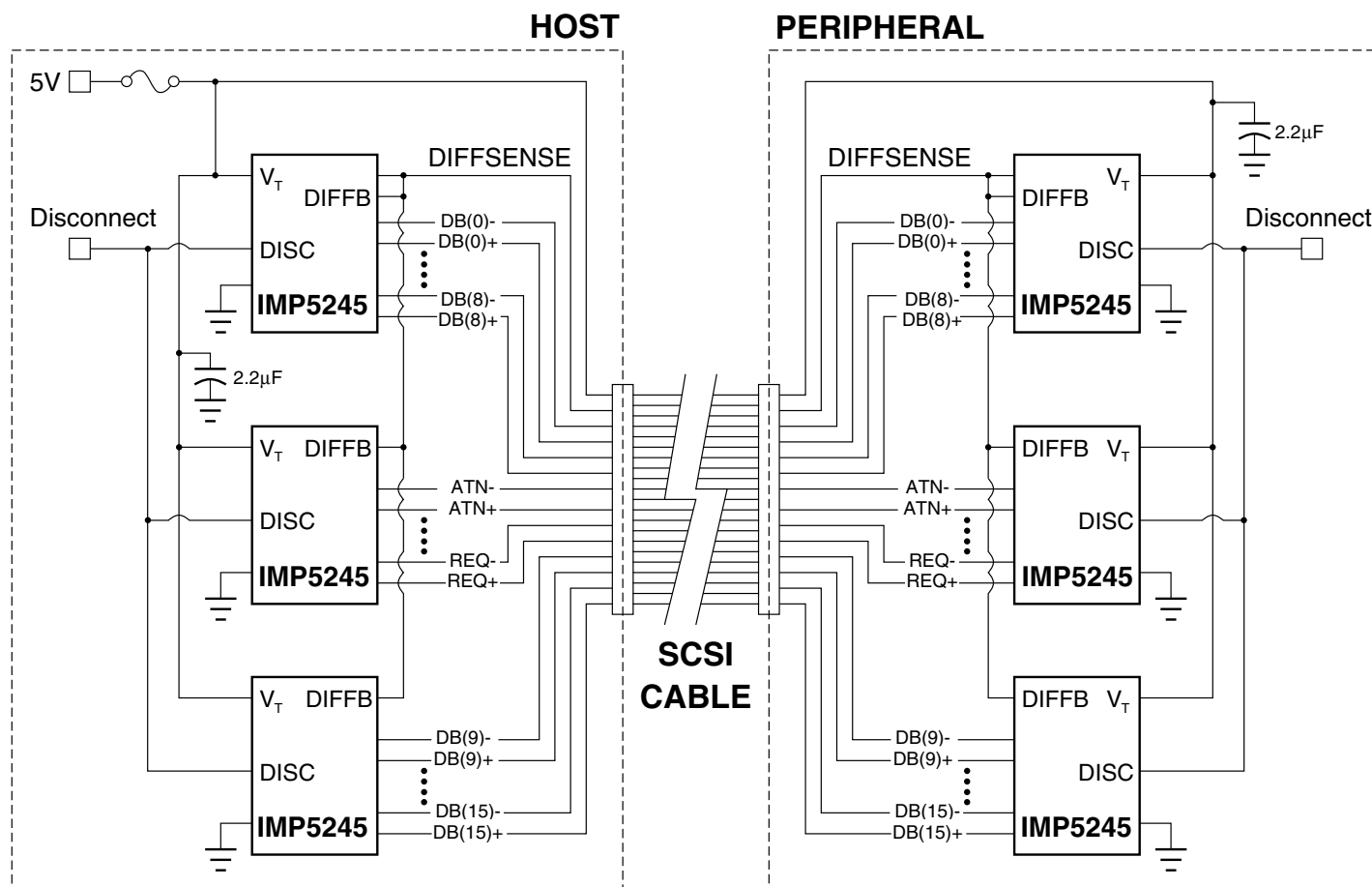
Figure 4. Application Schematic
