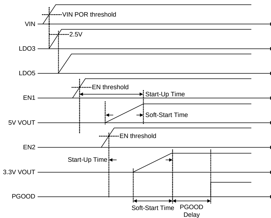
Figure 6. RT6545B Timing
