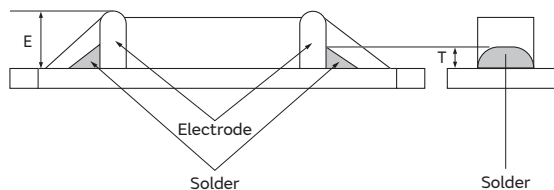
Reference: Optimum Solder Amount
