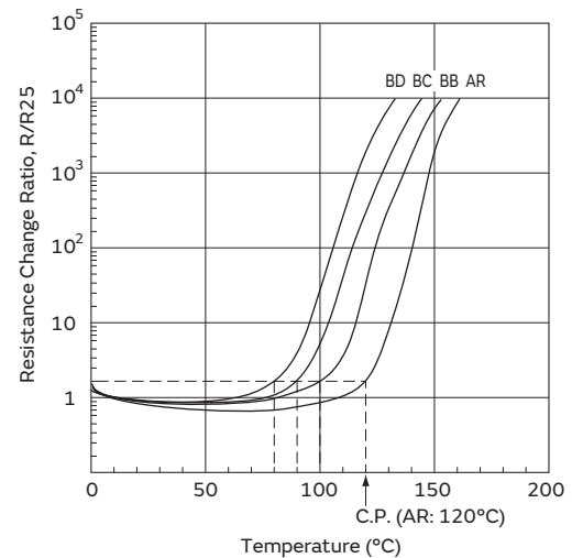
Resistance-Temperature Characteristic
