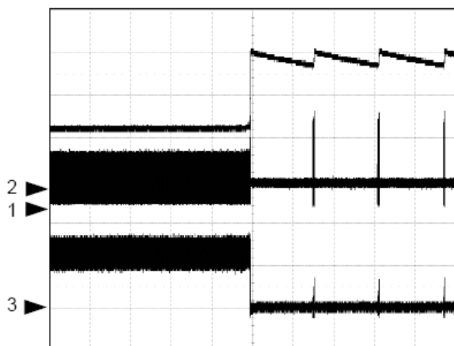
OPEN-LED Protection
