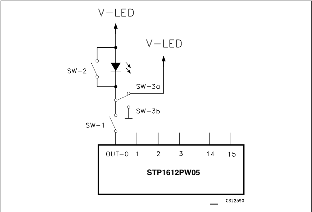
Figure 11. Detection circuit
