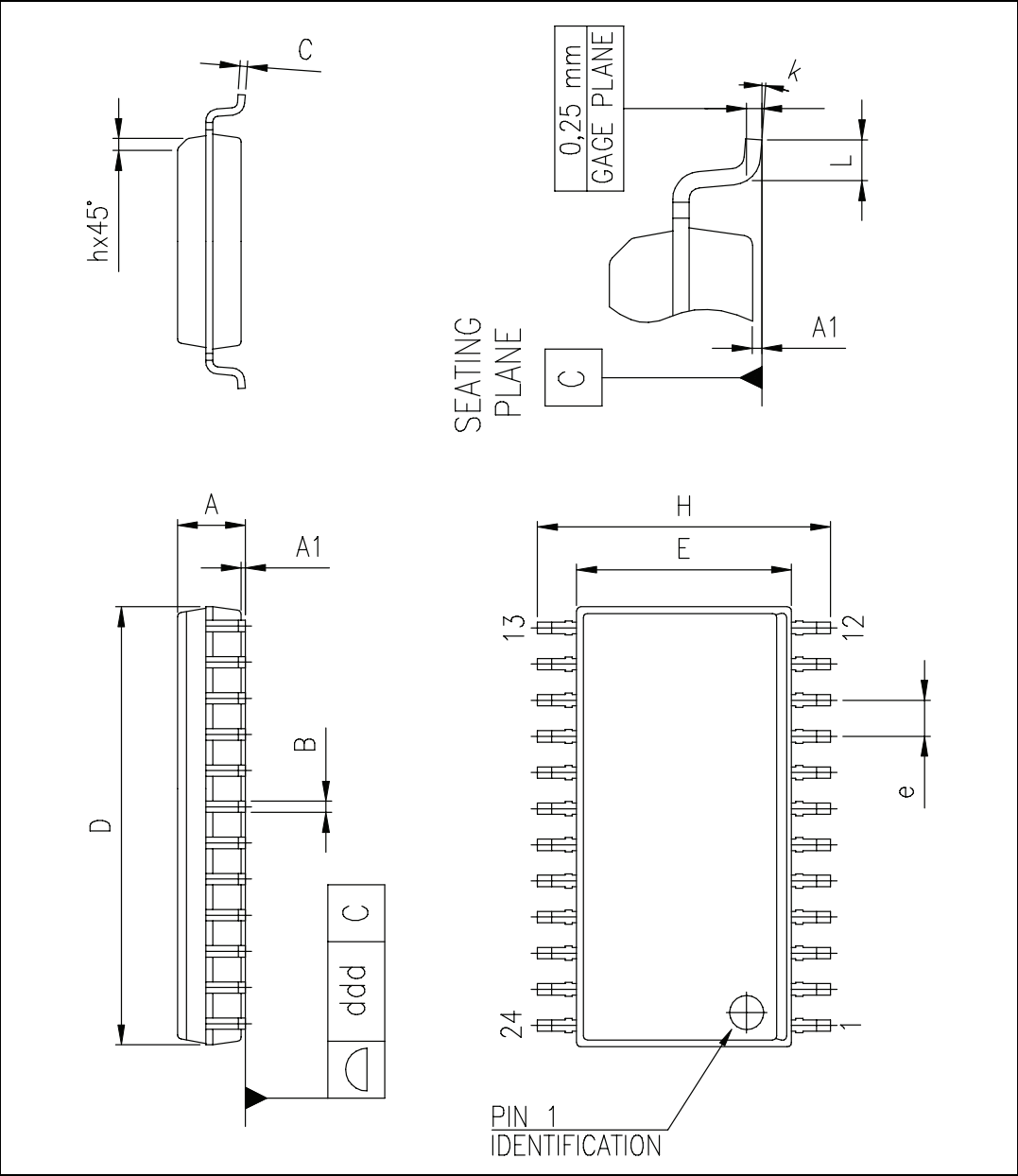
Figure 17. SO-24 package dimensions
