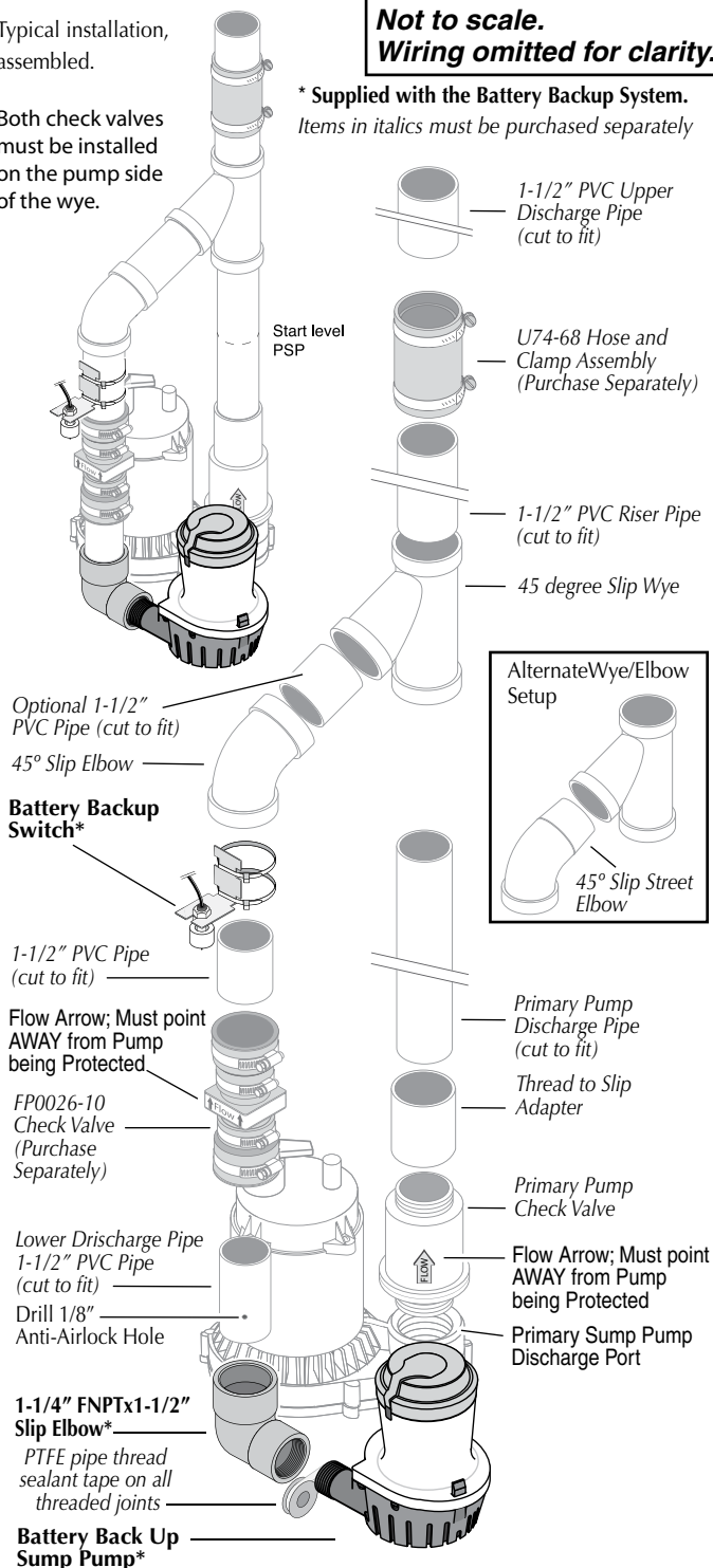
Figure 3: Typical installation with common discharge pipe.
