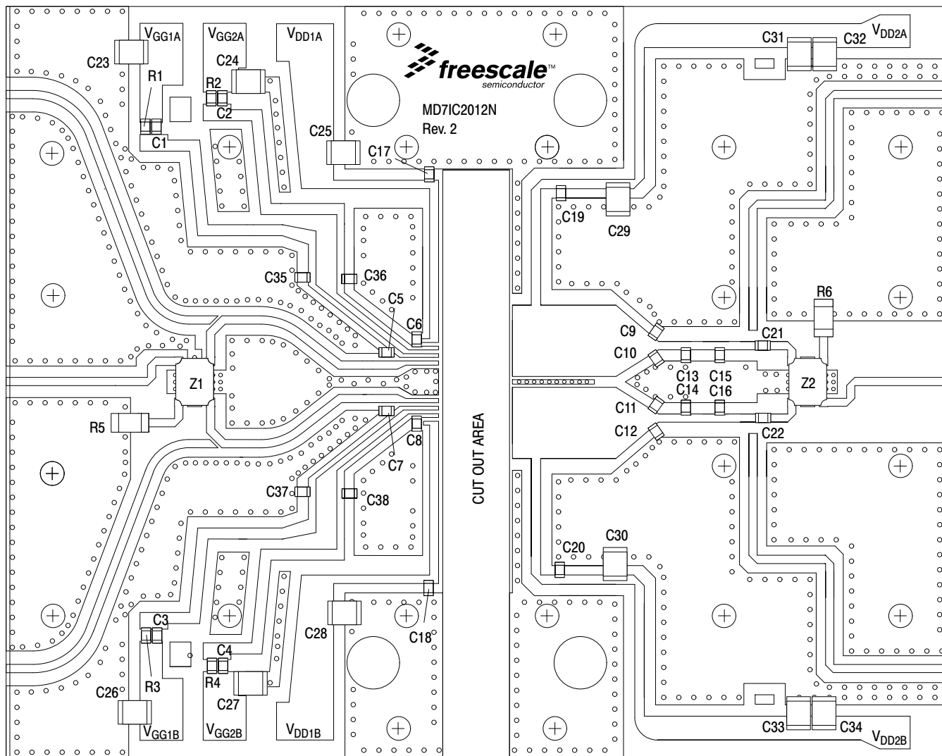
Figure 3. MD7IC2012NR1 Test Circuit Component Layout — 1805–2170 MHz
