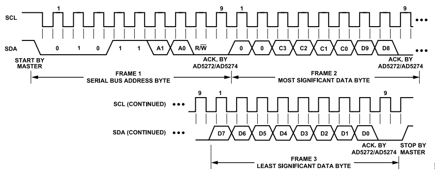
Figure 43. Write Command
