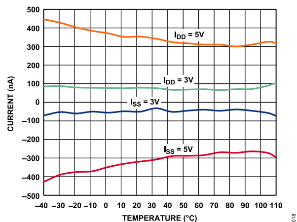
Figure 22. Supply Current ( I_{DD} , I_{SS} ) vs. Temperature
