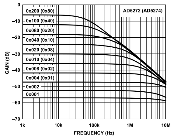
Figure 28. 100 kΩ Gain vs. Code vs. Frequency
