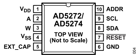
Figure 4. MSOP Pin Configuration
