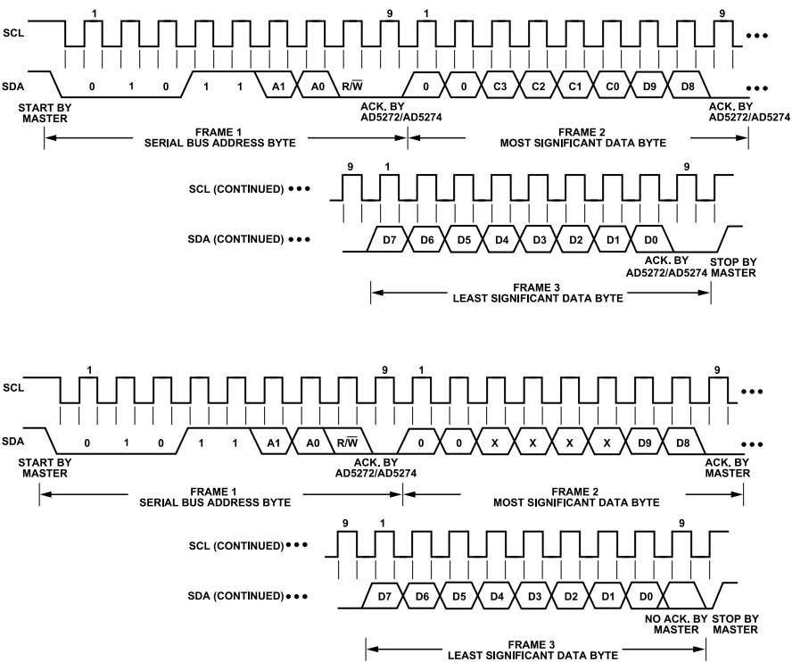
Figure 45. Read Command
