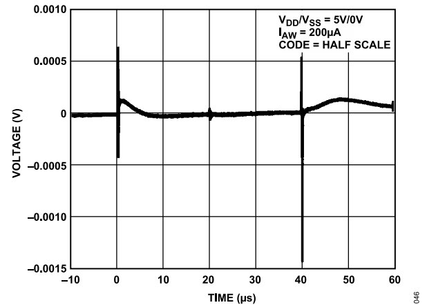
Figure 35. Digital Feedthrough
