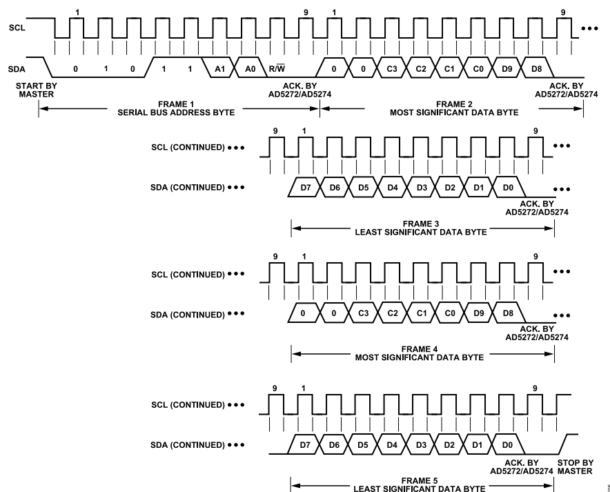
Figure 44. Multiple Write
