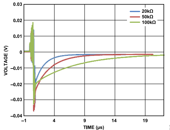
Figure 32. Maximum Glitch Energy
