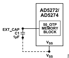
Figure 47. EXT_CAP Hardware Setup
