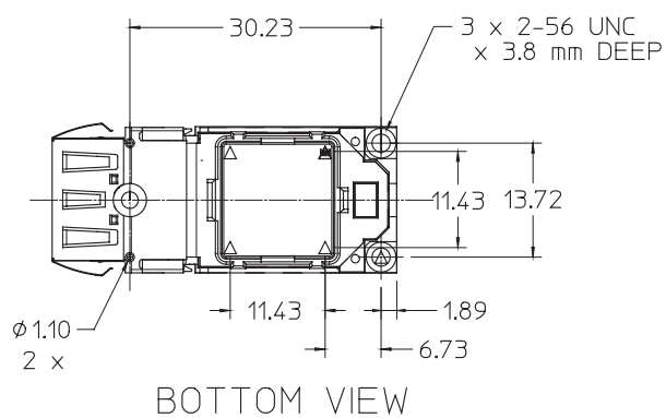
Figure 17. Package Outline for HFBR-779BEWZ and HFBR-789BEZ (dimensions in mm)
