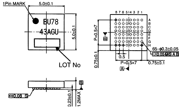
VBGA063T050 (Unit: mm)
