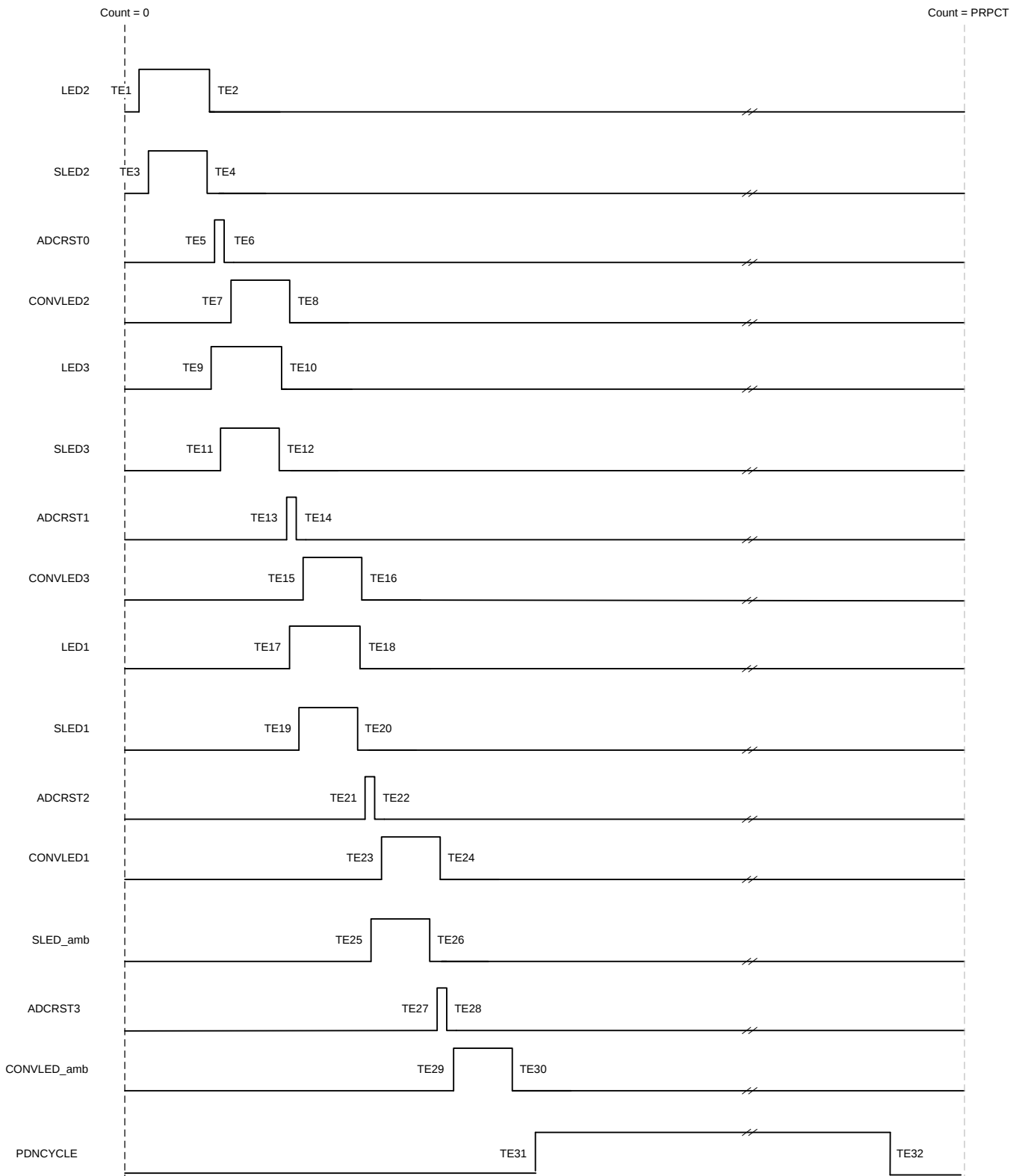
Figure 32. Timing Diagram
