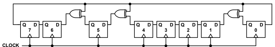
Figure 45. 8-Bit LFSR
