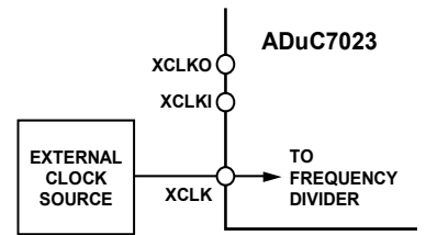
Figure 52. Connecting an External Clock Source
