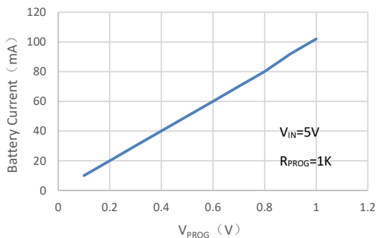
Battery Current vs. V_{PROG}
