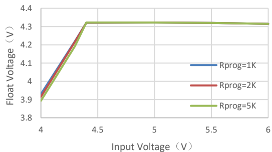
Float Voltage vs. Input Voltage (4.35V)
