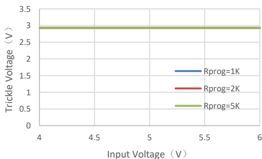
Trickle Voltage vs. Input Voltage
