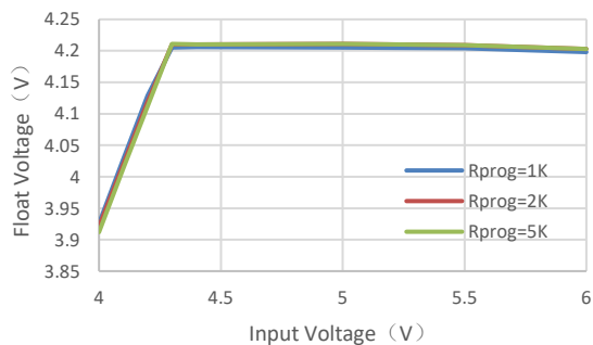
Float Voltage vs. Input Voltage (4.2V)
