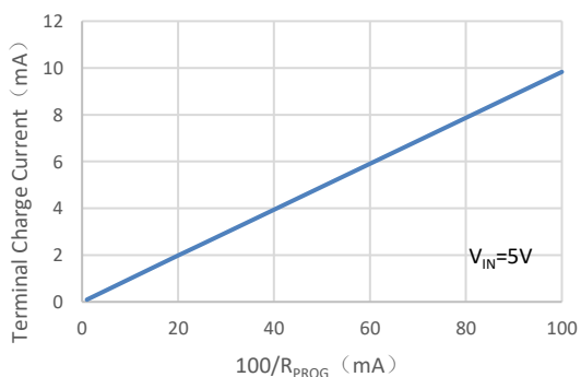
Terminal Charge Current vs. R_{PROG}
