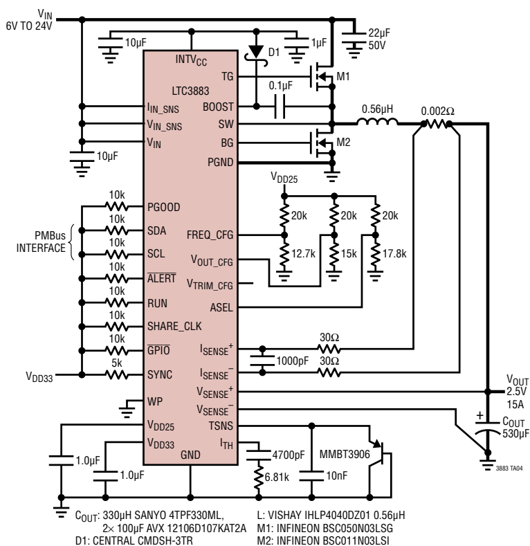
High Efficiency 500kHz 2.5V Step-Down Converter with Sense Resistor, No Input Current Sense
