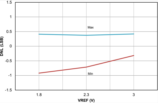
Figure 41-8. ADC, Single-Ended DNL, V_{DD} = 3.0V , T_{AD} = 1\mu S
