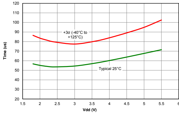
Figure 41-101. Wake From Sleep, VREGPM = 1, HFINTOSC = 4MHz
