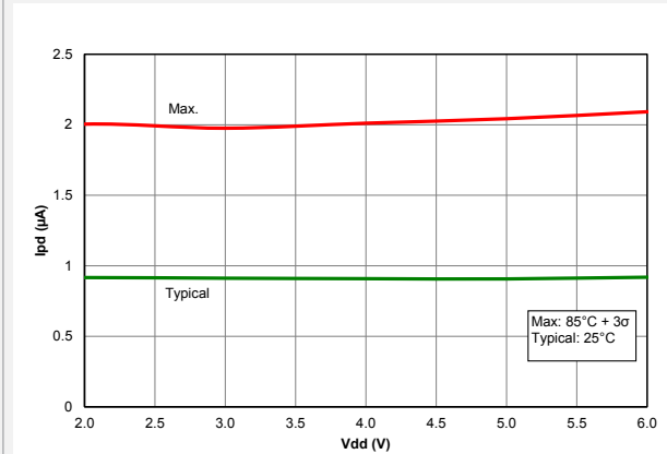
Figure 41-62. I_{PD} , Watchdog Timer, PIC18F65/66K40 only
