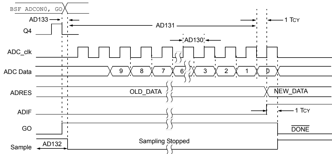
Figure 40-11. ADC Conversion Timing (ADC Clock from ADCRC)
