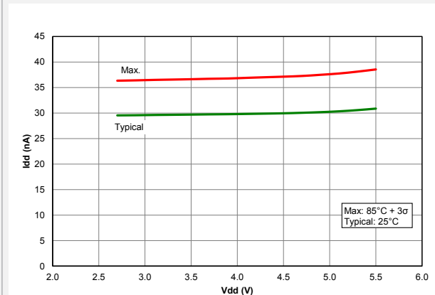
Figure 41-64. I_{DD} , Fixed Voltage Reference (FVR), PIC18F65/66K40 only
