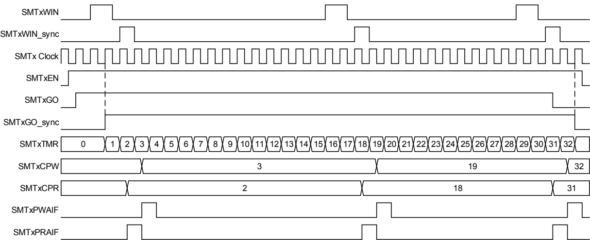
Figure 26-16. Capture Mode, Single Acquisition Timing Diagram
