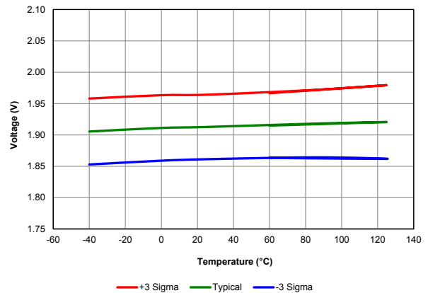
Figure 41-19. Brown-Out Reset Voltage, Trip Point (BORV = 11) for PIC18LF65/66K40 only
