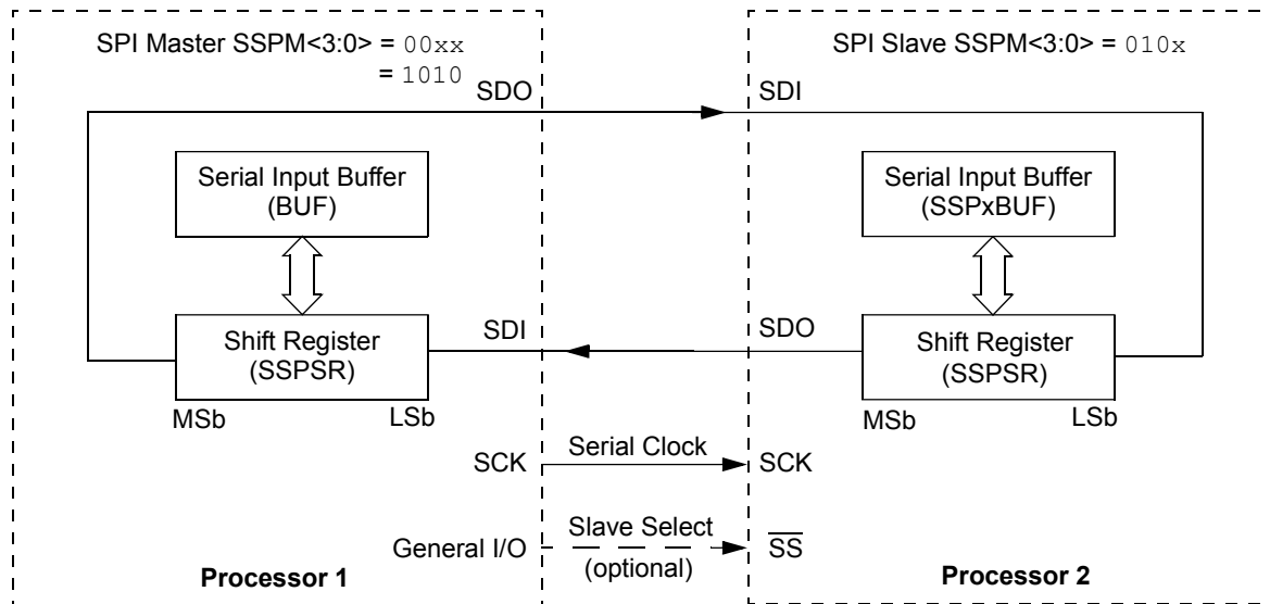
Figure 28-3. SPI Master/Slave Connection
