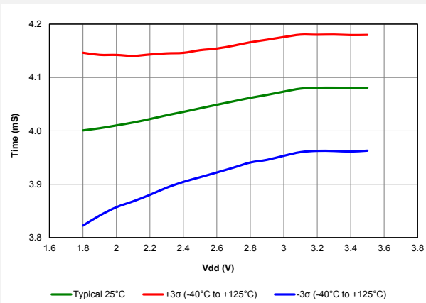
Figure 41-107. Watchdog Timer Time-out Period, PIC18LF65/66K40 only
