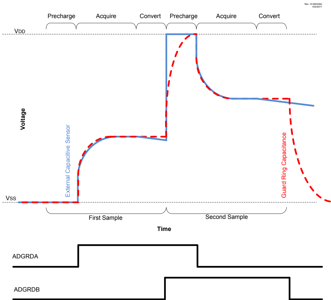
Figure 33-10. Hardware CVD Sequence Timing Diagram
