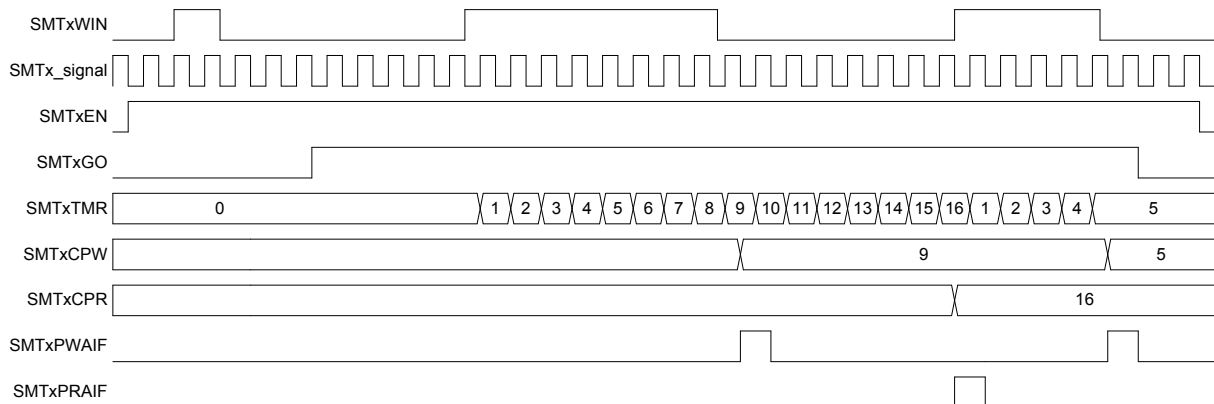
Figure 26-21. Windowed Counter Mode, Single Acquisition Timing Diagram
