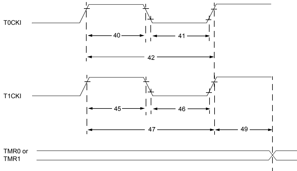
Figure 40-12. Timer0 and Timing1 External Clock Timings
