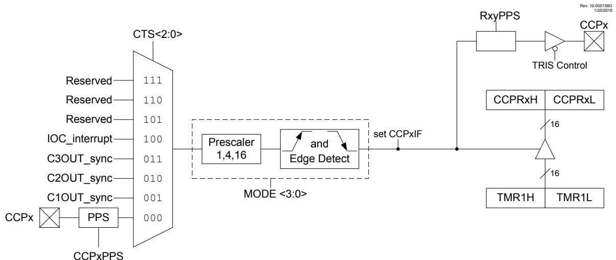
Figure 22-1. Capture Mode Operation Block Diagram
