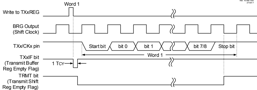
Figure 29-11. Synchronous Transmission
