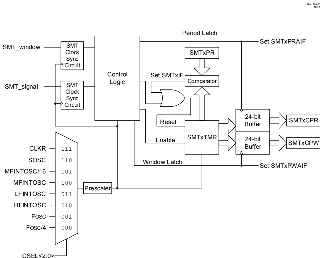
Figure 26-1. Signal Measurement Timer Block Diagram
