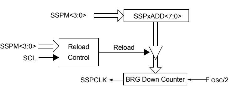
Figure 28-40. Baud Rate Generator Block Diagram
