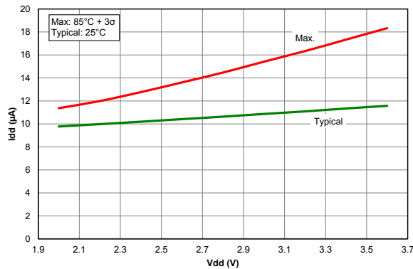
Figure 41-67. I_{PD} , Low-power Brown-out Reset, LPBOR = 0, PIC18LF65/66K40 only
