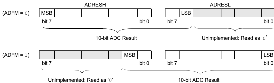
Figure 33-3. 10-Bit ADC Conversion Result Format
