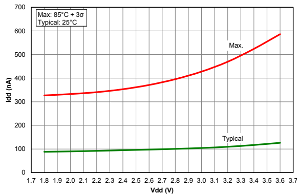
Figure 41-69. I_{PD} , Comparator, PIC18LF65/66K40 only
