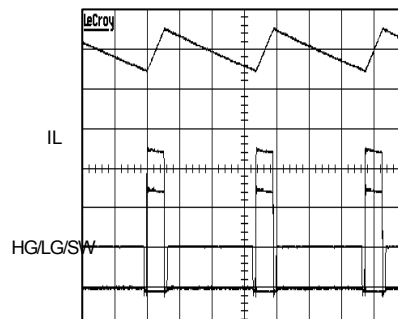
Fig.23 Continuous Mode ( I_o=4A )
