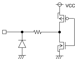
8pin (FS)
