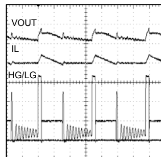
Fig.20 SLLM Mode ( I_{OUT}=0.4A )
