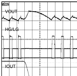
Fig.16 Transient Response ( V_{IN}=7V )
