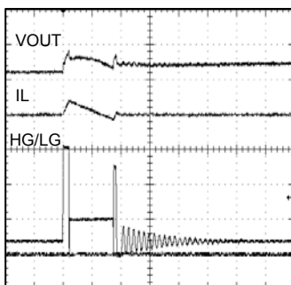
Fig.19 SLLM Mode ( I_{OUT}=0A )
