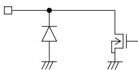
1pin (PGOOD)
