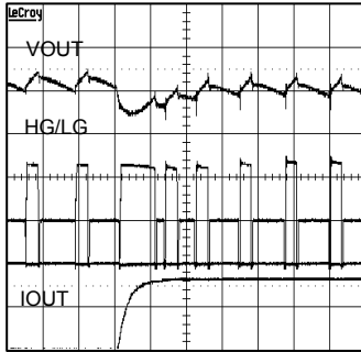
Fig.13 Transient Response ( V_{IN}=7V )
