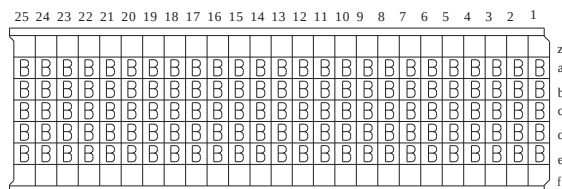
Board hole pattern (Component mounting side)
