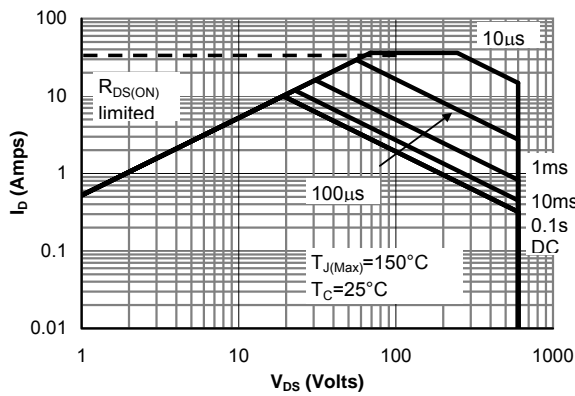
Figure 9: Maximum Forward Biased Safe Operating Area for AOT10N60 (Note F)
