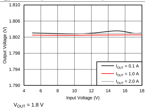
Figure 8. BUCK3, PSM Mode, Line Regulation
