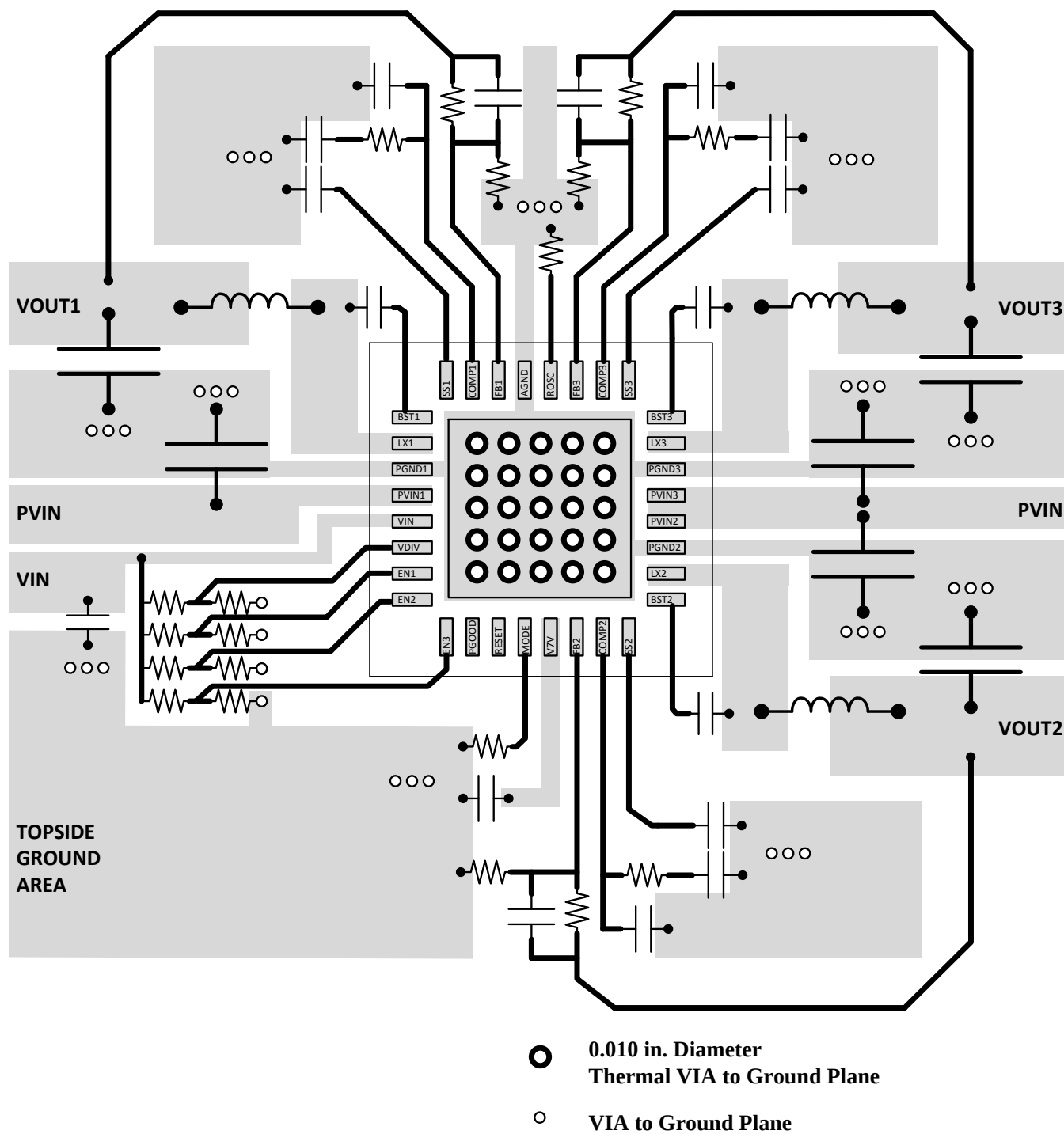
Figure 70. PCB Layout
