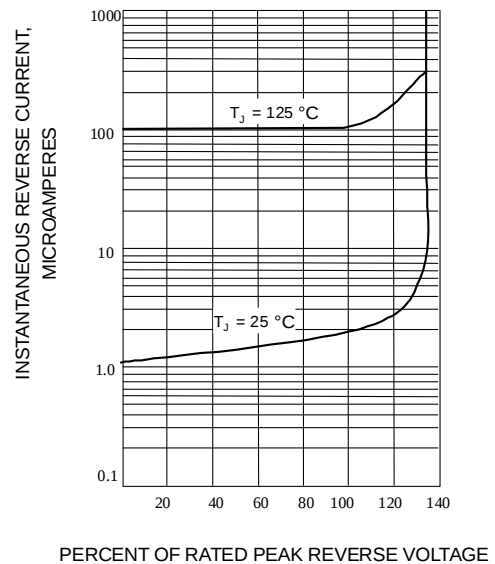
Fig. 2-TYPICAL REVERSE CHARACTERISTICS
