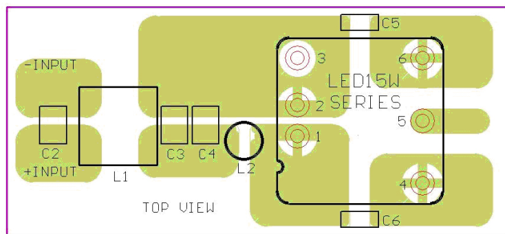
Recommended EN55022 Class B Filter Circuit Layout
