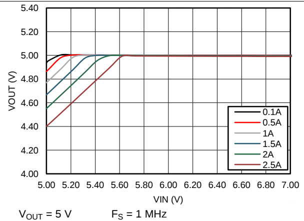
Figure 16. Dropout Curve
