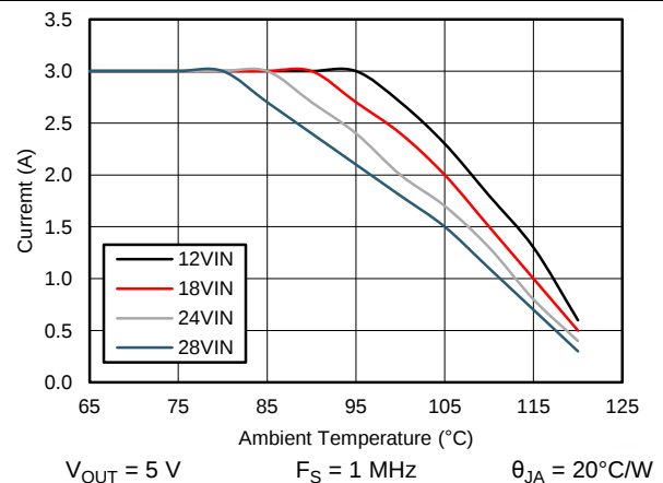
Figure 84. Derating Curve
