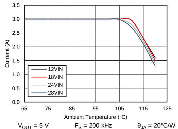
Figure 72. Derating Curve
