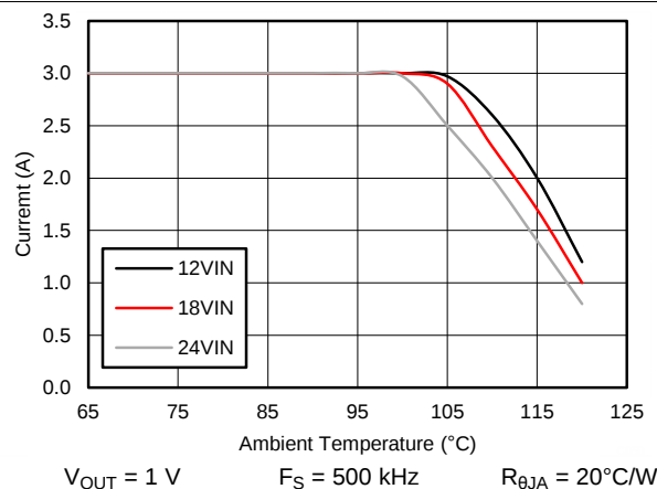
Figure 54. Derating Curve
