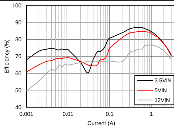
Figure 50. Efficiency
