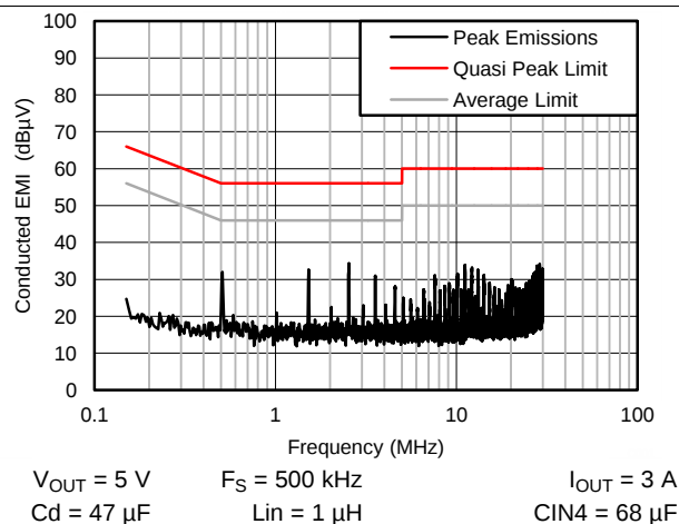
Figure 34. Conducted EMI Curve
