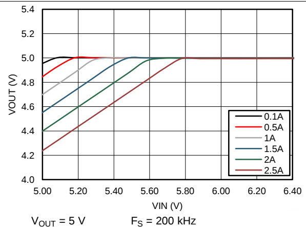
Figure 70. Drop-out Curve
