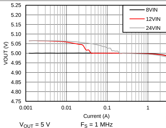
Figure 81. Output Voltage Regulation
