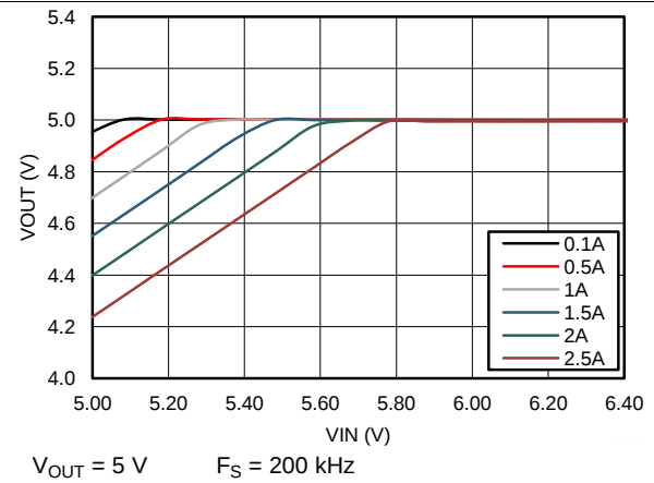
Figure 14. Dropout Curve
