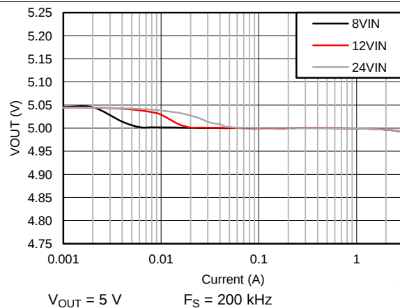
Figure 69. Output Voltage Regulation
