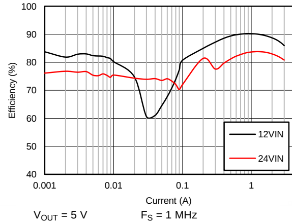
Figure 80. Efficiency
