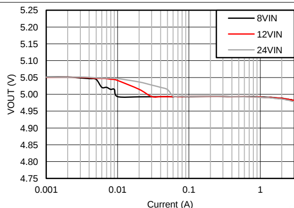
Figure 75. Output Voltage Regulation
