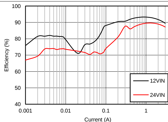
Figure 74. Efficiency at Room Temperature
