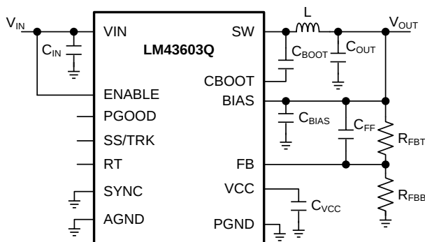
Figure 46. LM43603-Q1 Basic Schematic for V OUT ≥ 3.3 V, tie BIAS to V OUT
