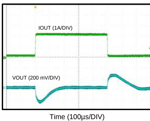
Figure 93. Output Voltage Regulation
