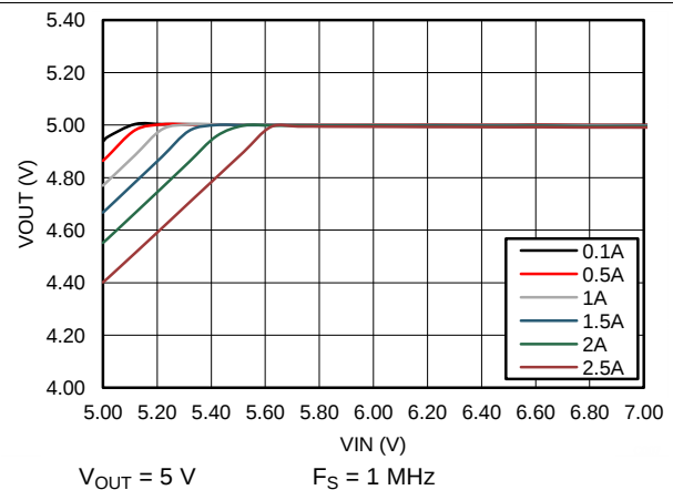
Figure 82. Drop-out Curve
