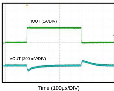
Figure 69. Output Voltage Regulation
