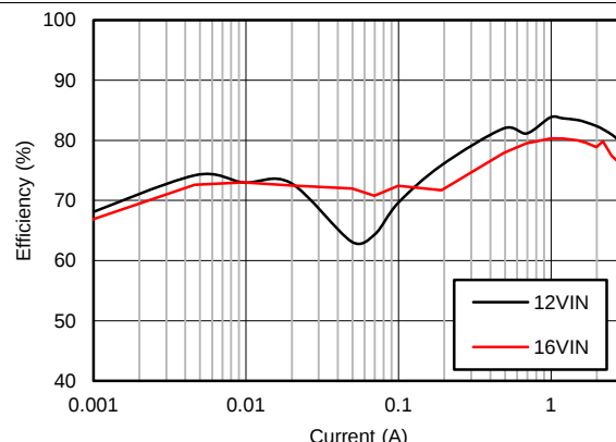
Figure 86. Efficiency
