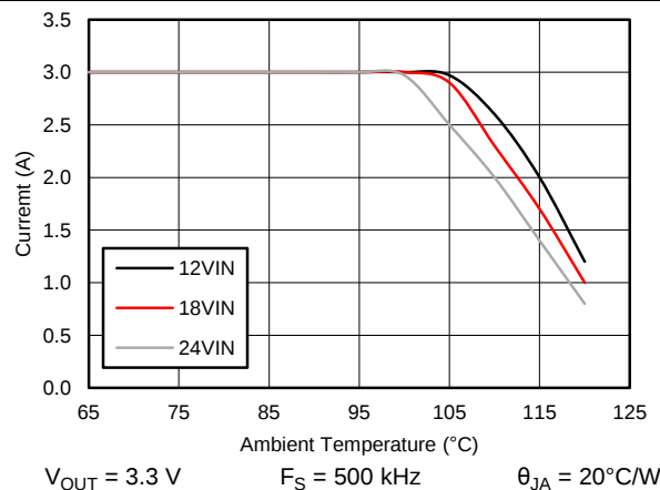
Figure 66. Derating Curve
