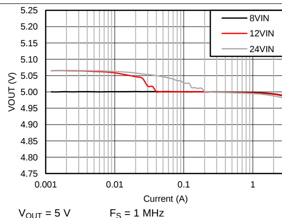
Figure 10. V_{OUT} Regulation
