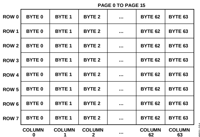
Figure 35. EEPROM Page Diagram
