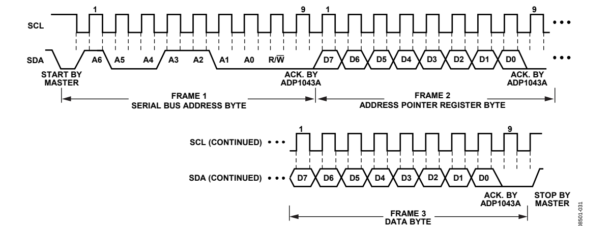
Figure 32. Writing a Register Address to the Address Pointer Register, and Then Writing Data to the Selected Register
