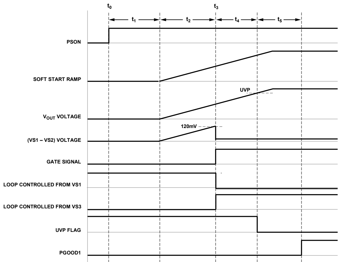
Figure 21. Soft Start Timing Diagram
