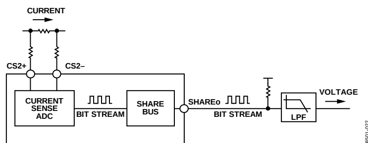
Figure 23. Analog Current Share Configuration
