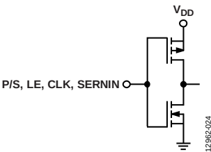
Figure 6. P/S, LE, CLK, and SERNIN Interface
