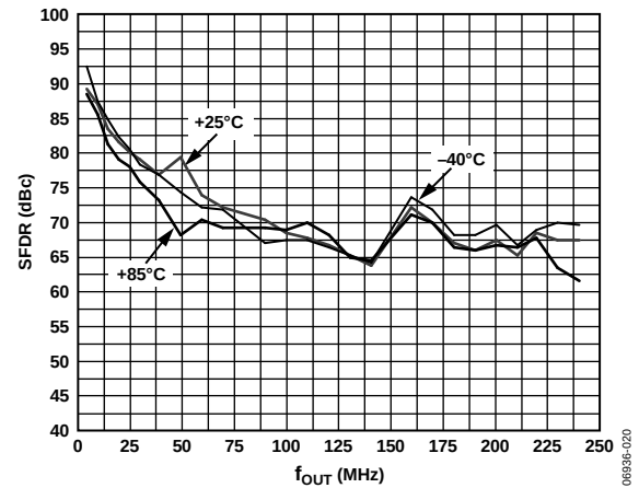
Figure 20. AD9783 SFDR vs. f_{OUT} Over Temperature, at 500 MSPS, FS = 20 mA
