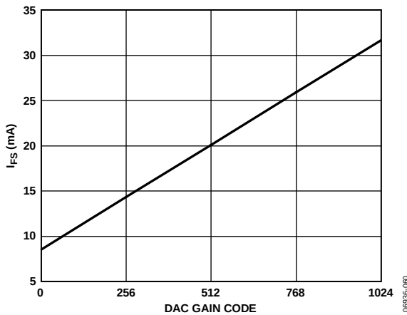
Figure 63. I_{\text{FS}} vs. DAC Gain Code
