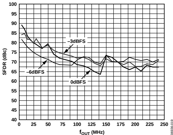
Figure 19. AD9783 SFDR vs. f_{OUT} Over Digital Input Level, T_A = 25^\circ\text{C} , at 500 MSPS, FS = 20 mA
