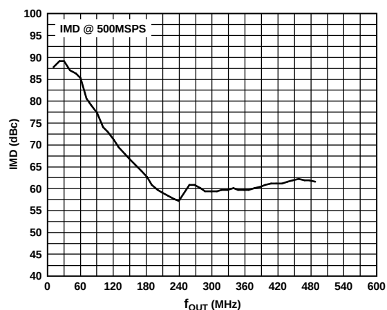
Figure 42. AD9781 IMD vs. f_{OUT} in Baseband and Mix Modes, at 500 MSPS, FS = 20 mA
