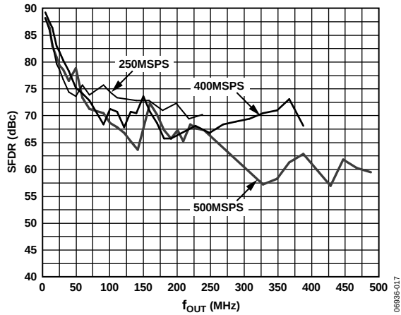
Figure 17. AD9783 SFDR vs. f_{OUT} Over f_{DAC} in Baseband and Mix Modes, FS = 20 mA
