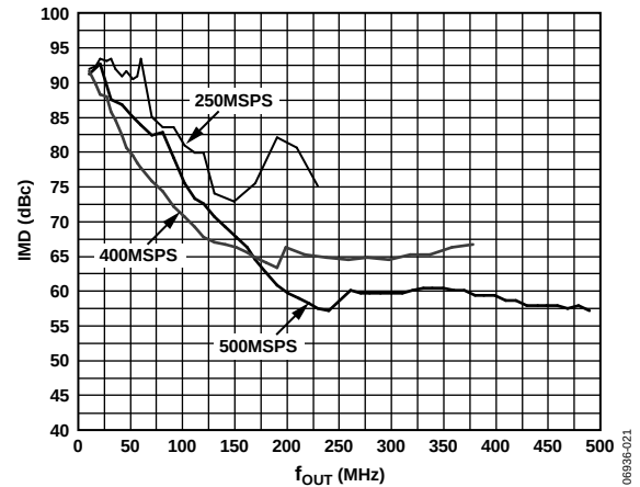
Figure 21. AD9783 IMD vs. f_{OUT} Over f_{DAC} in Baseband and Mix Modes, FS = 20 mA
