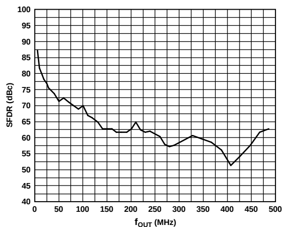
Figure 41. AD9781 SFDR vs. f_{OUT} in Baseband and Mix Modes, at 500 MSPS, FS = 20 mA
