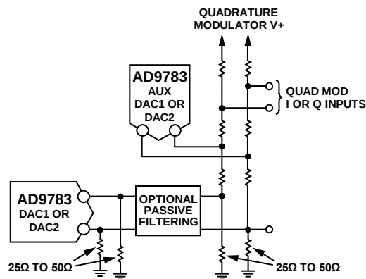
Figure 67. DAC DC-Coupled to Quadrature Modulator with a Passive DC Shift
