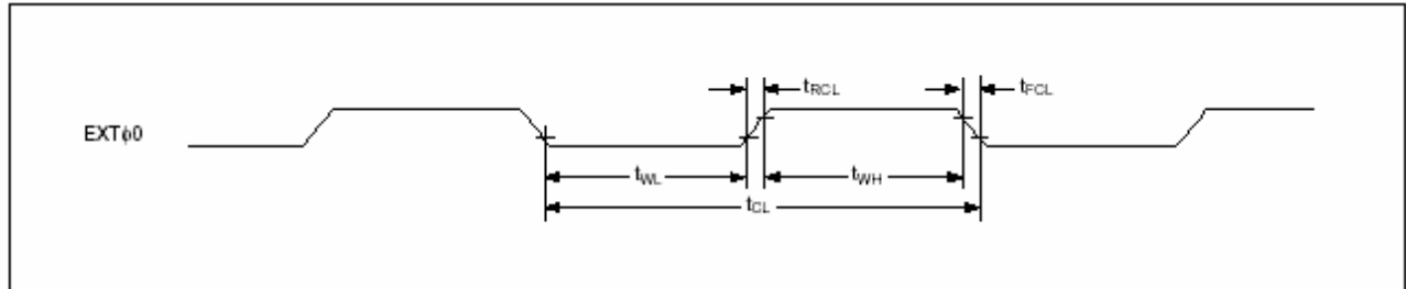
External oscillator signal timing
